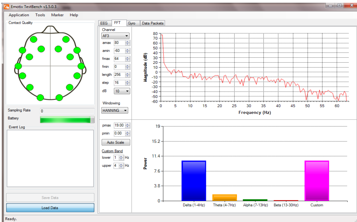
Figure 9: FFT Measurements in TestBench. TestBench also measures Delta, Theta, Alpha, Beta, and a user-defined custom band.
