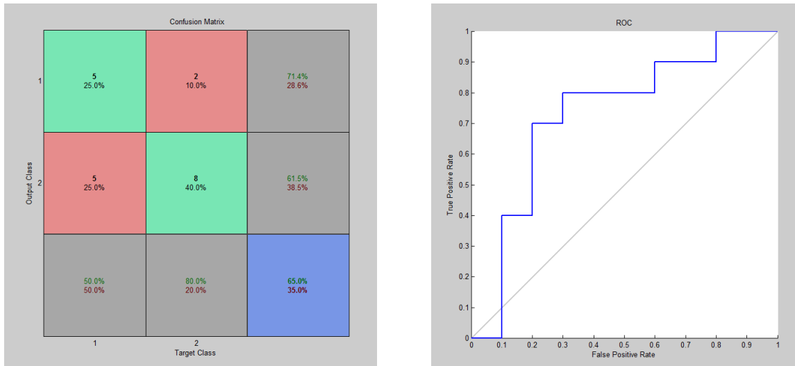
Figure 15: Initial Neural Net Results showing both a Confusion Matrix and Receiver Operating Characteristic (ROC) Plot
