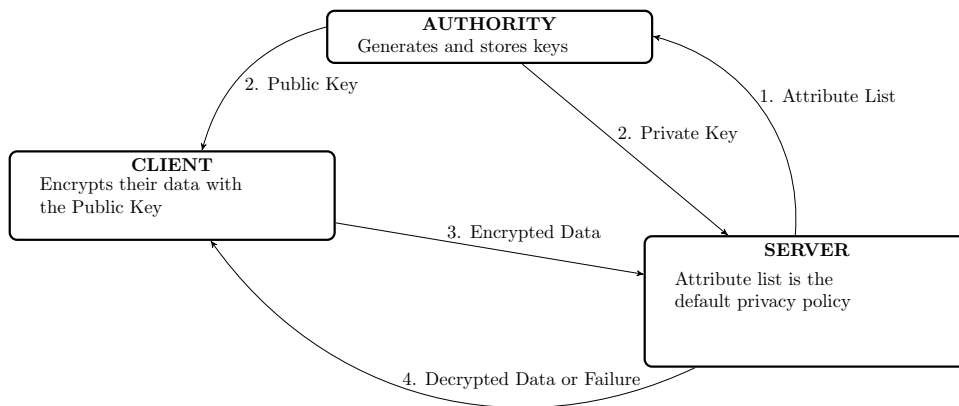
Figure 2: Prototype encryption/decryption process
