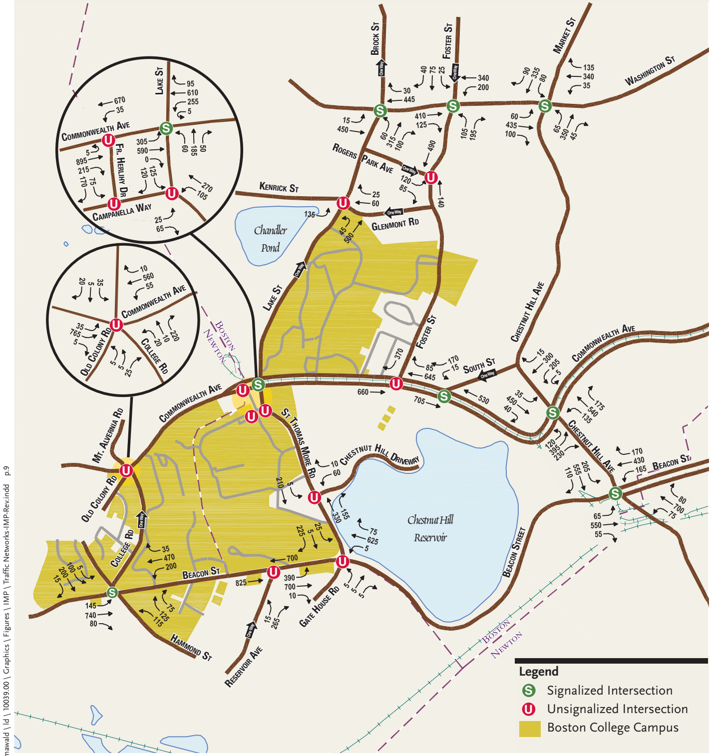
No-Build Condition Morning Peak Hour Traffic Volumes Study Area Intersections
