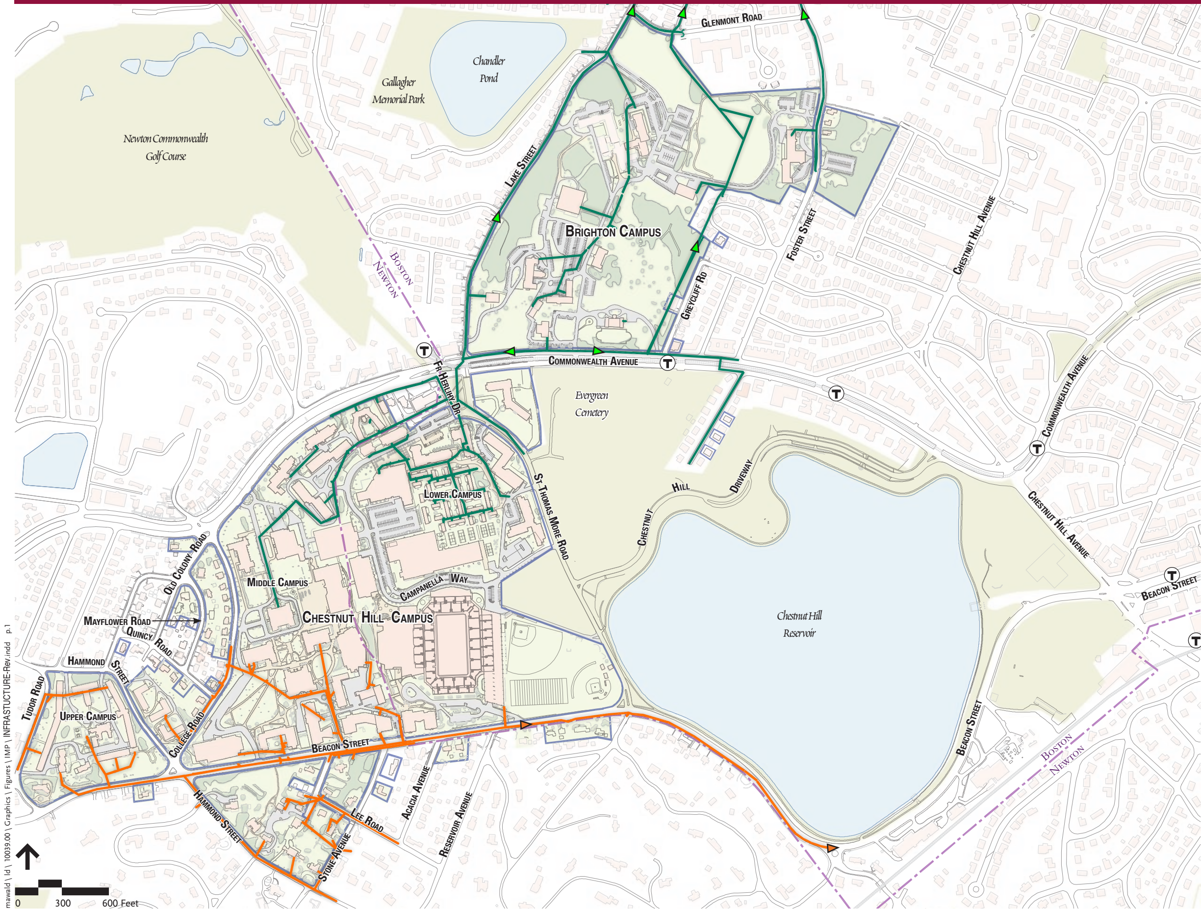
Figure 8-1 Existing Sanitary Sewer System Boston College Institutional Master Plan
