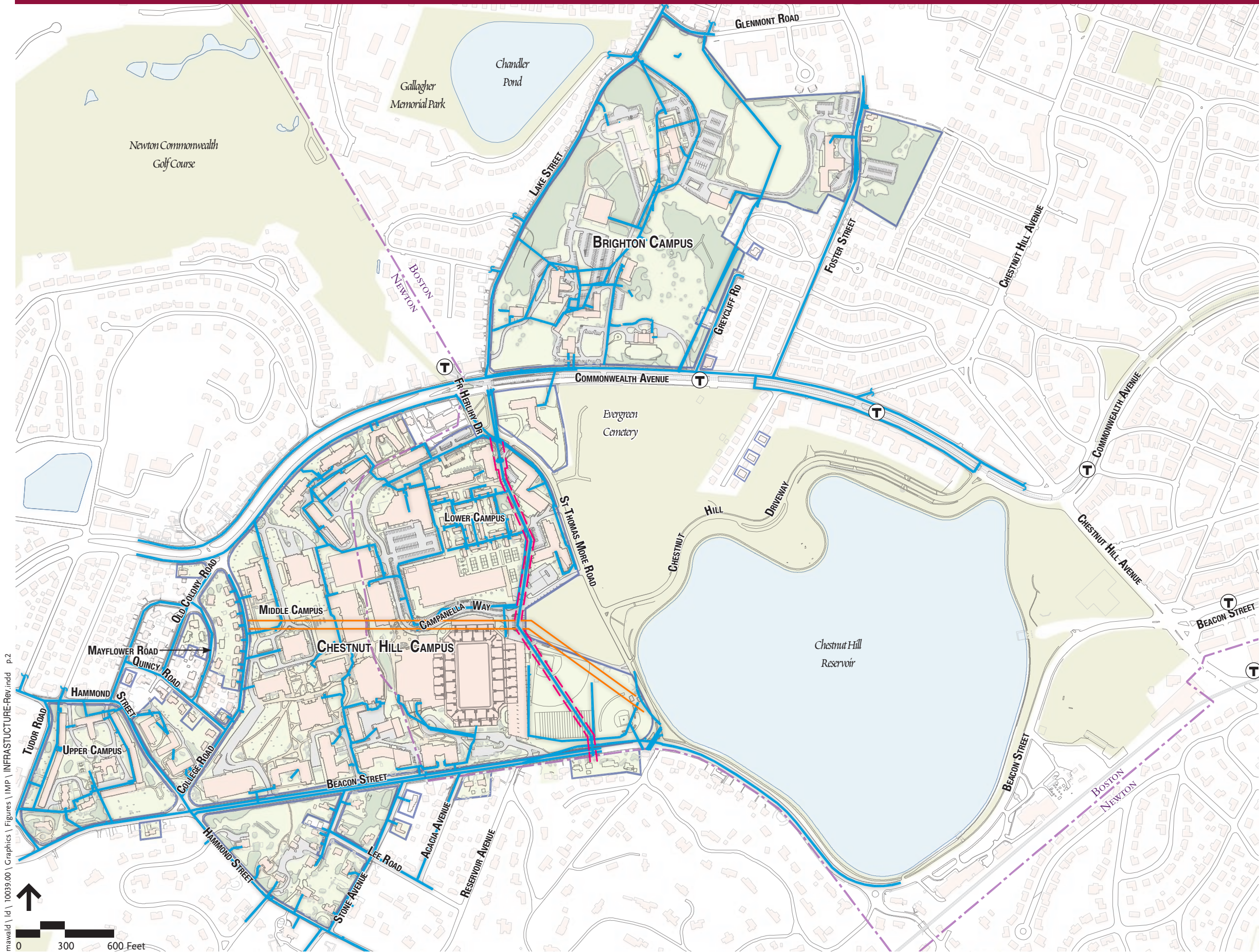
Figure 8-2 Existing Water Supply System
