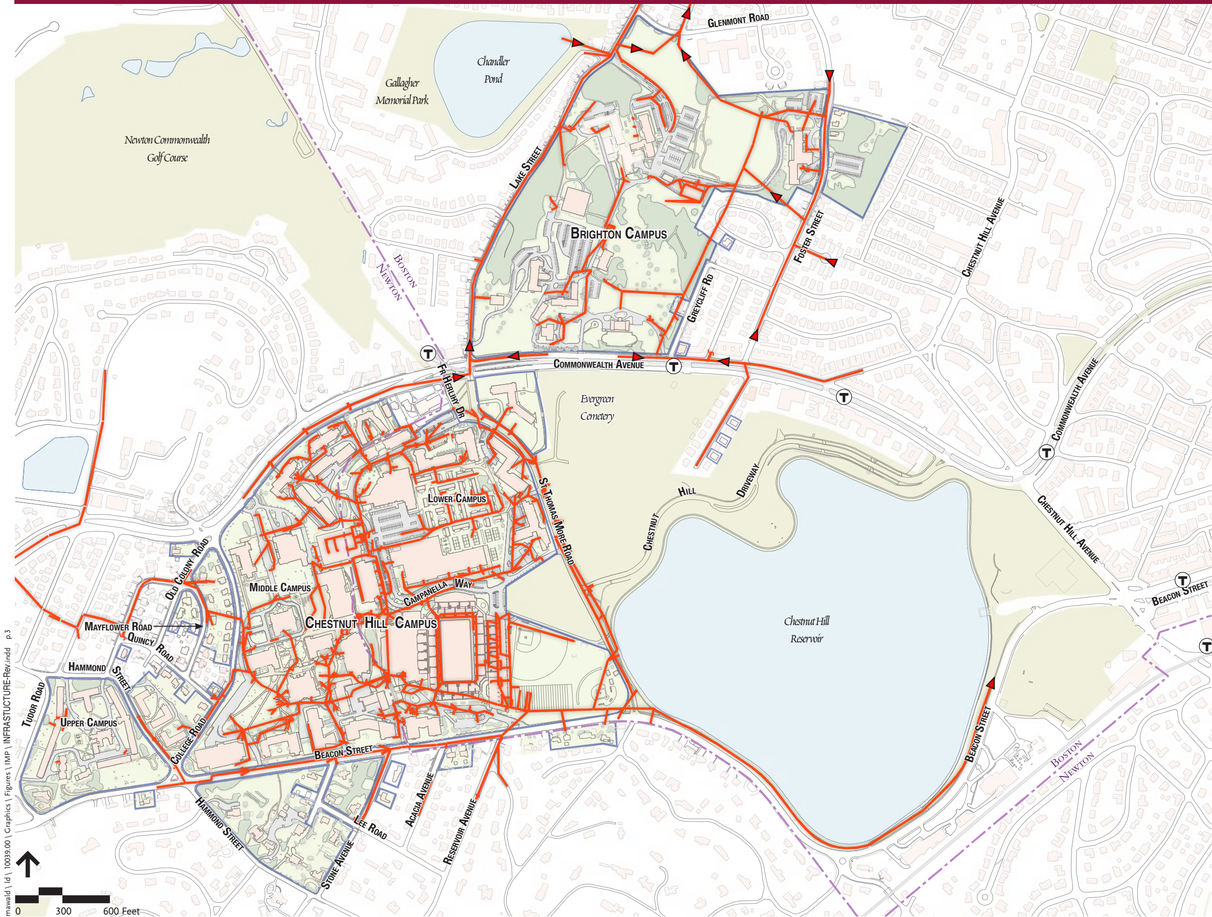
Figure 8-3 Existing Stormwater System Boston College Institutional Master Plan
